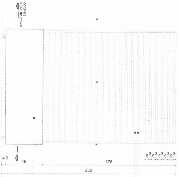
VISTA FRONTAL
